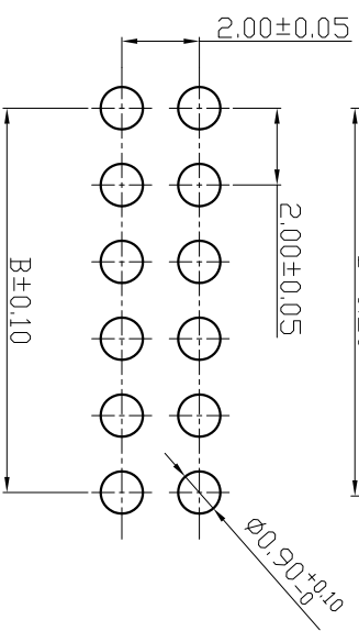
PCB Layout
